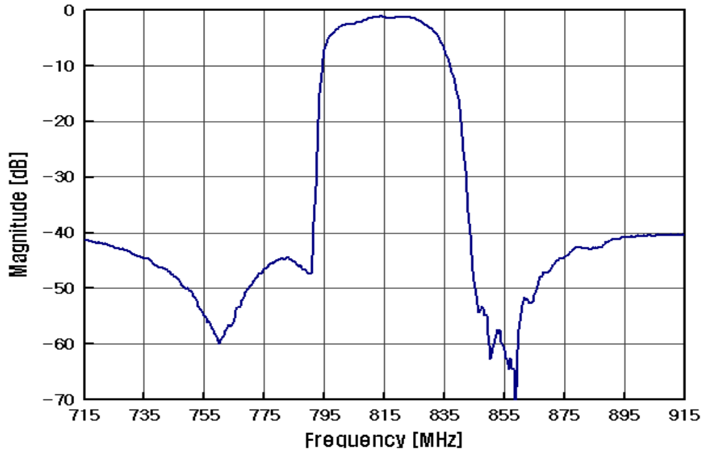
Frequency Response
